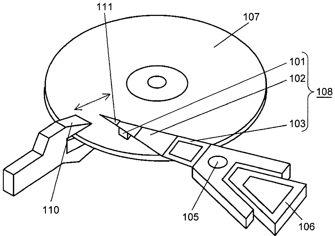
FIG. 10 – PRIOR ART
